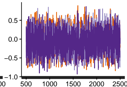
tau[3]
