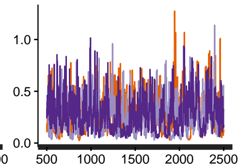
tau[1]
