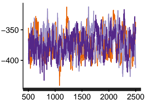
log-posterior
