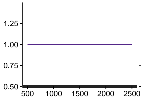
Omega[3,3]
