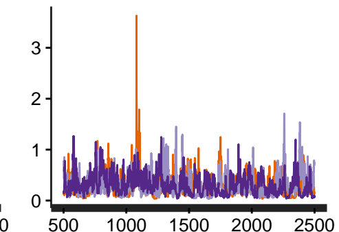
tau[2]
